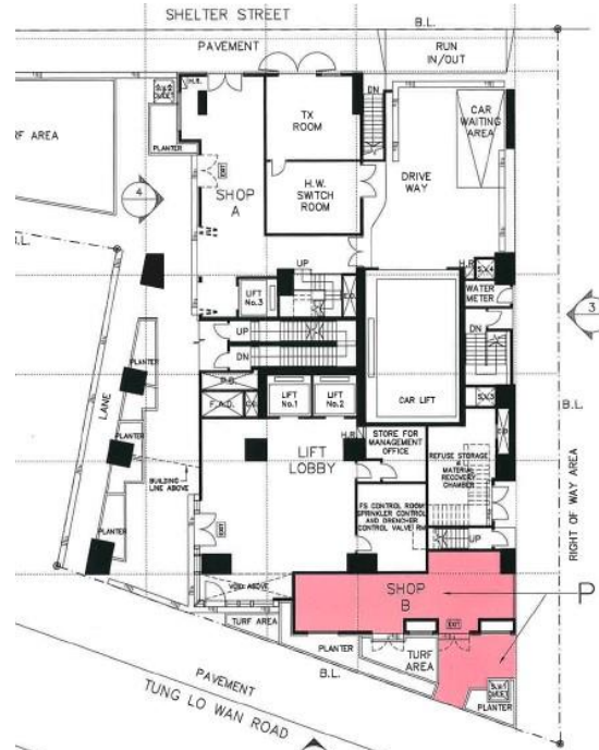
YOO RESIDENCE GROUND FLOOR PLAN NOT TO SCALE FOR REFERENCE ONLY
